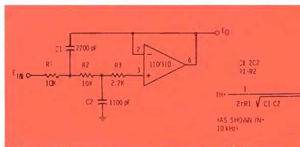
Fig. 5a Low-pass filter has unity gain in passband, rolls off 12dB/octave above cutoff.
