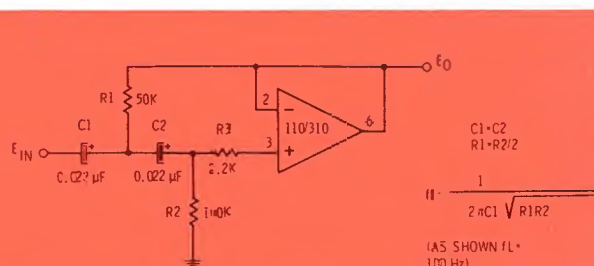
Fig. 5b High-pass filter has unity gain in passband, rolls off 12dB/octave below cutoff.
