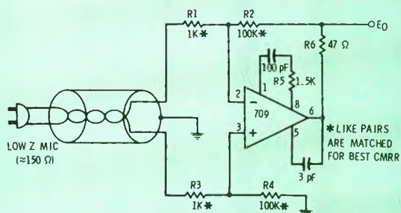
Fig. 1a Transformerless differential input microphone preamp.
