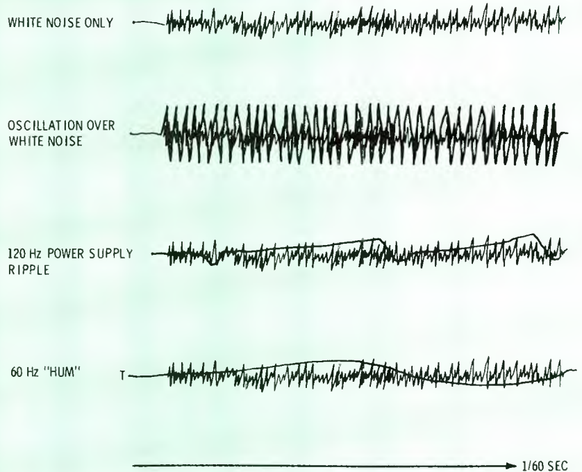
Fig. 2 Typical system noise outputs are shown graphically for clarity. A combination of these noises can be difficult to interpret. A high gain audio amplifier is sometimes a useful tool in identifying the type of noise so that its source may be found.
