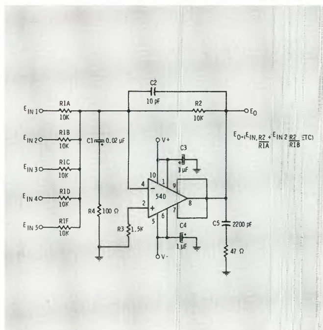
Fig. 3 Summing amplifier combines multiple inputs without loss.
