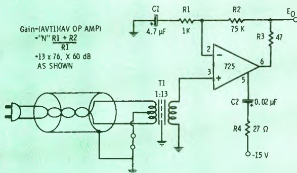
Fig. 1b Transformer input microphone preamp.
