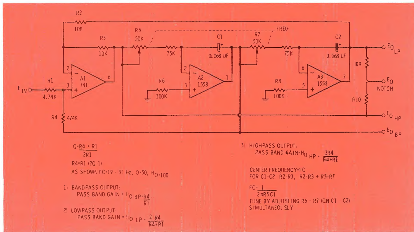
Fig. 5c Variable filter "does everything": HP, LP, BP, and notch with high gain and Q.
